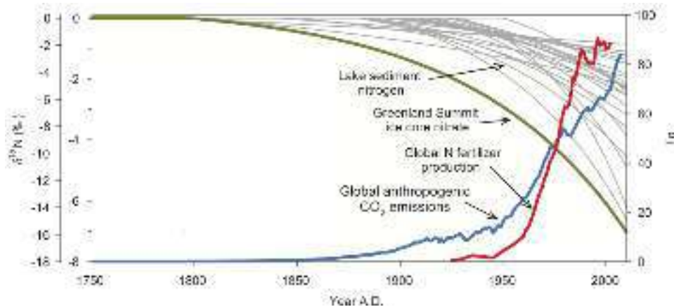
Figure 12. Relative changes in d^{15}N isotope ratios in sediments from 25 Northern Hemisphere lakes over the past 260 years (inner left ordinate), standardized to a common asymptotic value. Also shown is the relative change in d^{15}N-NO_3 from the Greenland Summit ice core (outer left ordinate), Haber-Bosch N fertilizer production (right ordinate), and global anthropogenic CO_2 emissions (right ordinate, data rescaled by 1/100 for plotting purposes). From Holgrieve et al. 2011.
