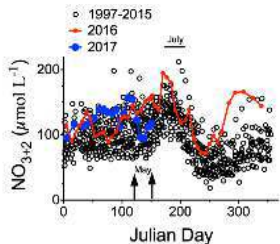
Figure 5. The concentration of nitrite+nitrate (NO 2+3 ) at Baton Rouge, LA from 1997 to present. Unpublished data from Turner et al.
