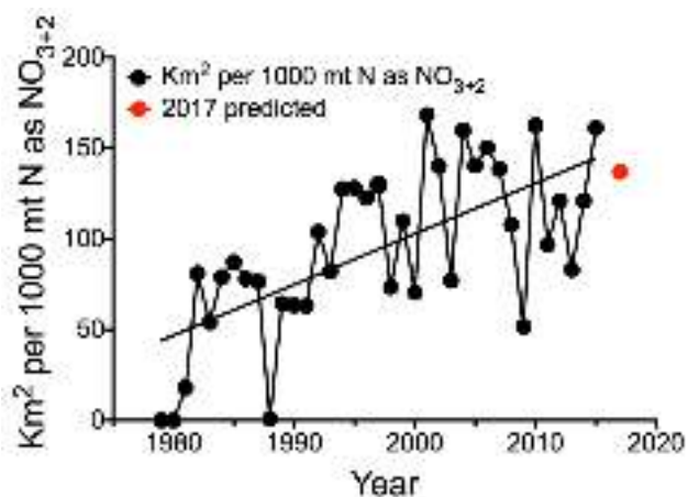
Figure 8. The size of the hypoxic zone per unit May nitrate loading. All years, including strong storm years, are included.
